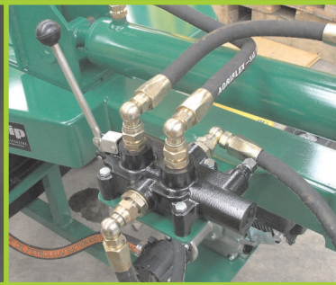
Valve bank c/w detent
